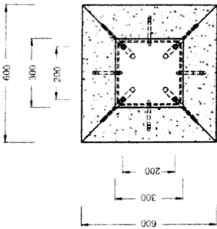
TOP VIEW SCALE 1:14
